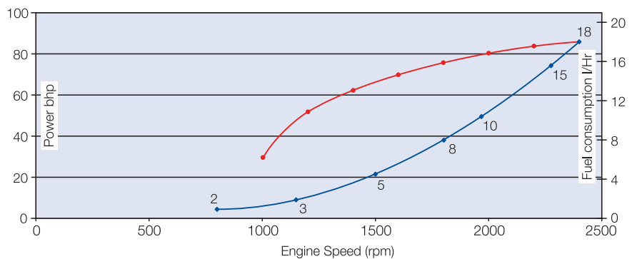
Propeller law consumption (2.8 index).
